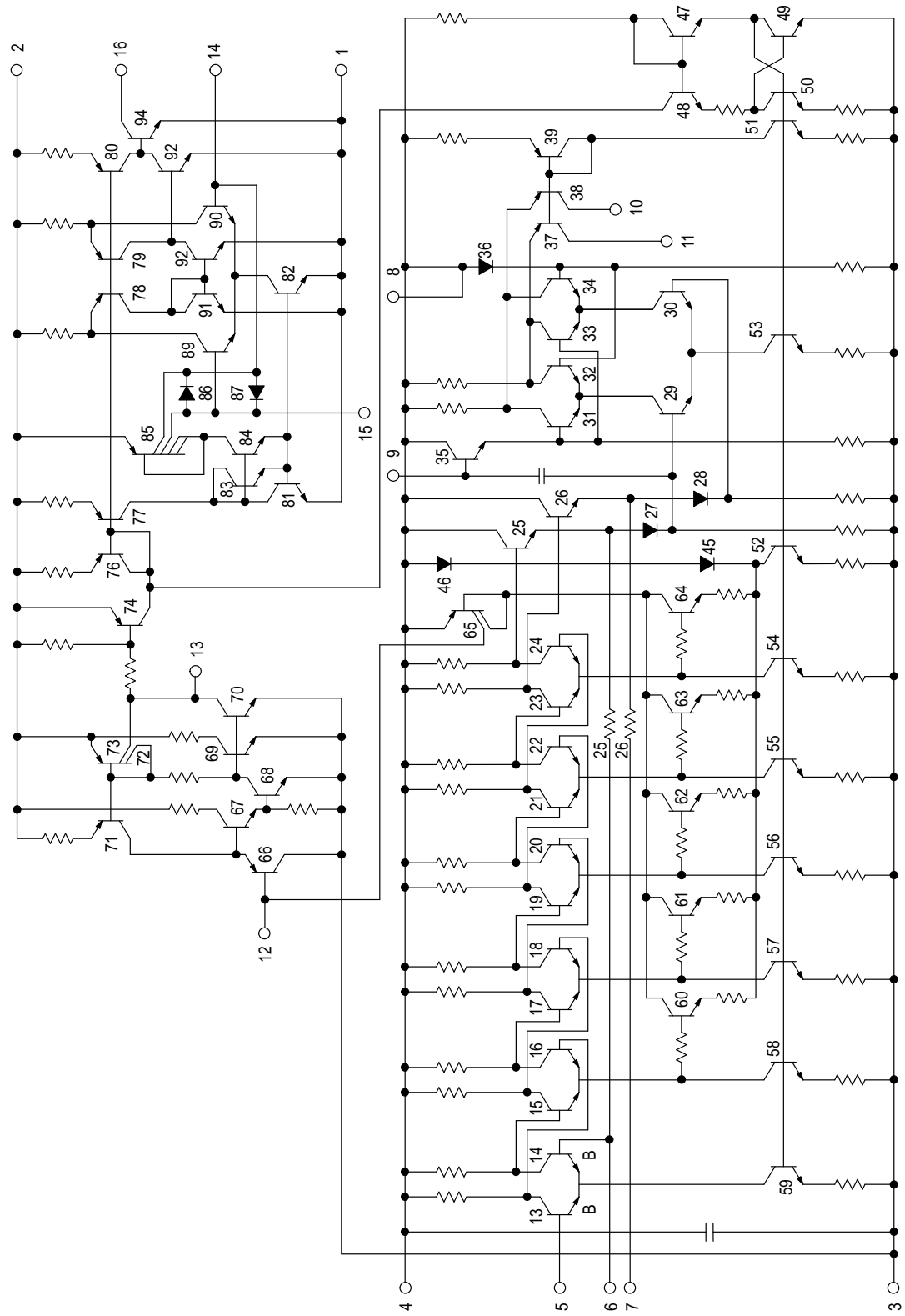
Figure 15. Internal Schematic
