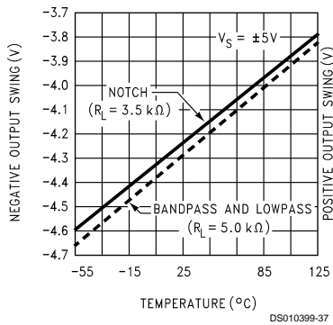
Negative Output Swing vs Temperature
