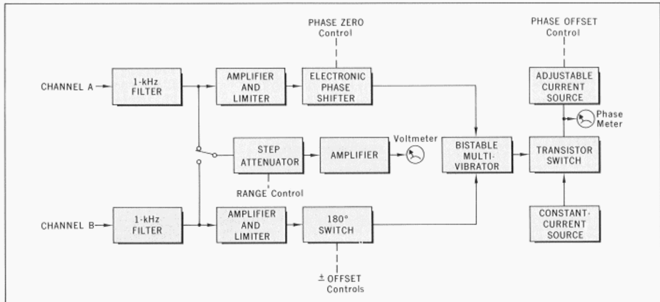
Fig. 9. Block diagram of voltmeter and phasemeter circuits. Amplifier-limiters make phase readings independent of signal levels.
