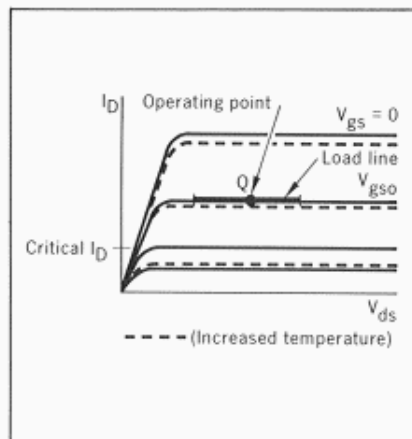
Fig. 4. Typical characteristic curves for field-effect transistor. Increase in temperature changes V_{gs} of load line to compensate for temperature-induced changes of operating points in associated bi-polar transistors.
