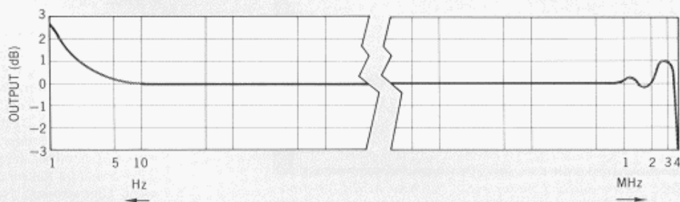
Fig. 1. Frequency response of new -hp- Model 427A Multi-func-
