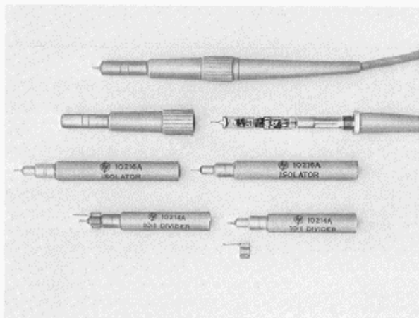
Fig. 10. Probes and accessories for -hp- Model 8405A Vector Voltmeter. Top to bottom: assembled probe; exploded view of probe, showing sampler circuit; isolators, 10:1 dividers, and ground clips supplied with probes. Isolators (or dividers) and ground clips are used when probing by hand in arbitrary circuits. (Tees and adapters are available for probing in 50-ohm coaxial systems.) Dividers extend upper limit of voltmeter range to 10 V. See Specifications for details.
