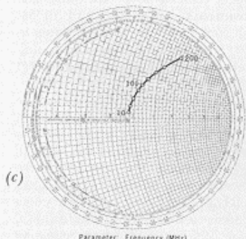
Expanded Smith chart plot of reflection coefficient of 50-ohm ±1% metal film resistor attached to
