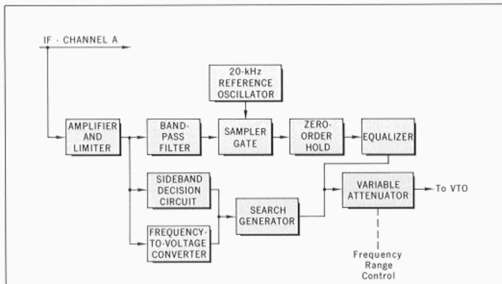
Fig. 8. Block diagram of automatic phase control (APC) circuit, which tunes and phase-locks Vector Voltmeter to channel A signal. APC loop adjusts frequency of voltage-tuned local oscillator (VTO) which generates sampling pulses for mixers, thus keeps IF at 20 kHz. APC requires only 10 ms to tune meter, and remains locked even if input frequency changes at rates up to 15 MHz/s. Sideband decision circuit ensures that f_{sig} - nf_{VTO} is always +20 kHz, never -20 kHz.
