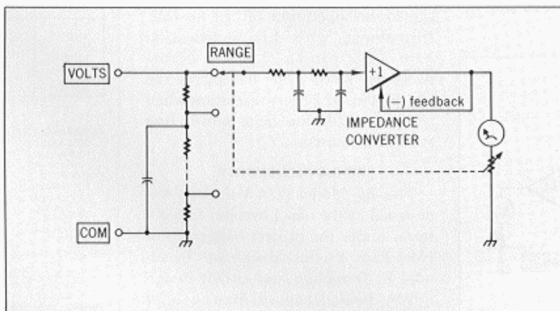
Fig. 6. Block diagram of new multi-function meter in dc voltage
