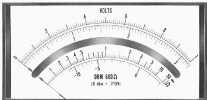
Fig. 3. Each mirror-backed meter scale for new Multi-function Meter is individually calibrated on -hp-'s servo-controlled meter calibrator. Meter face, shown here three-fourths actual size, also includes dB scale calibrated for 600 ohm systems. Meter has
