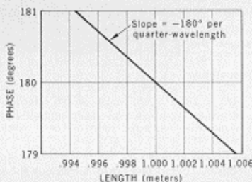
Phase versus length of cable for system shown in block diagram, calibrated at 75 MHz (quarter-
